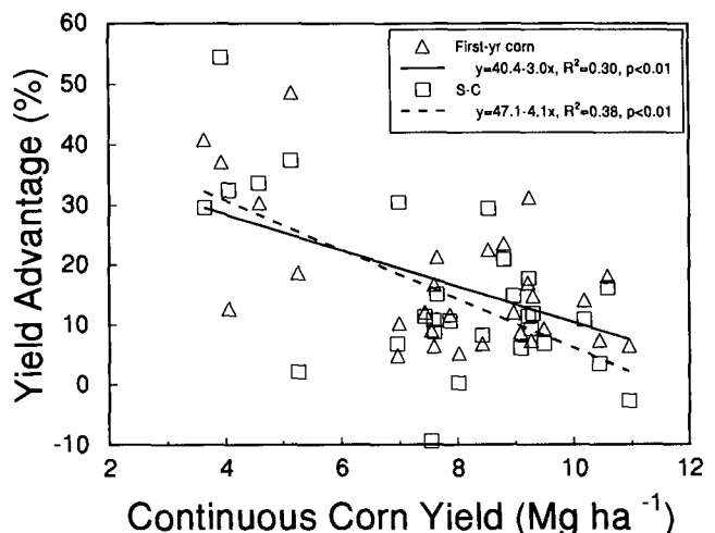
Fig. 3. Relationship between the yield advantage of corn in a soybean-corn (S-C) rotation and 1st-yr corn after 5 yr of soybean compared with continuous corn for 29 environments.
