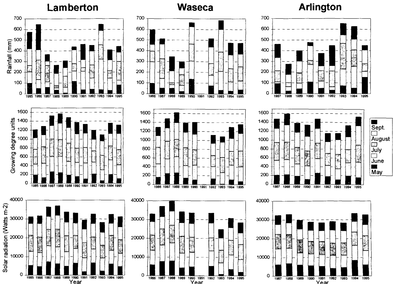
Fig. 1. Monthly rainfall, growing degree units, and solar radiation at Lamberton, MN, Waseca, MN, and Arlington, WI, from corn planting through September. Growing degree units were calculated each day as [(T_{max} - T_{min})/2] - T_{base} , where 10^{\circ}C \leq T_{max} and T_{min} \leq 30^{\circ}C and T_{base} = 10^{\circ}C .
