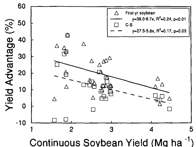
Fig. 5. Relationship between the yield advantage of soybean in a corn-soybean (C-S) rotation and 1st-yr soybean after 5 yr of corn compared with continuous soybean for 28 environments.
